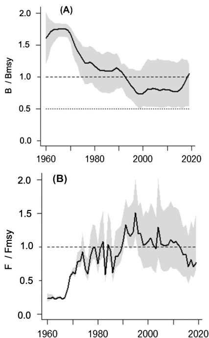
Fig. 3. A, Relative stock size ( B/B_{msy} ); and B, Relative fishing pressure ( F/F_{msy} ) per year.
